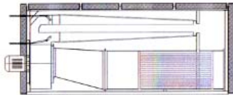
Rear view of air channel
